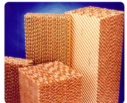
The steeper angle directs more water to the air entering side of the pad where it is needed the most.
